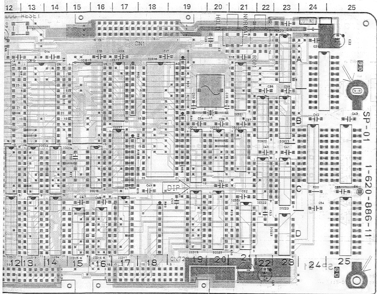
1-620-886-11 SOLDER SIDE
